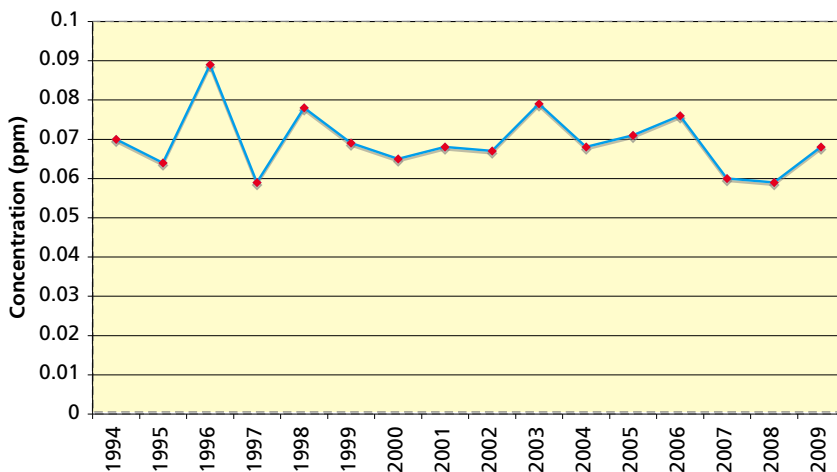
Yearly 8 Hour Ozone Levels: 4th highest concentration
