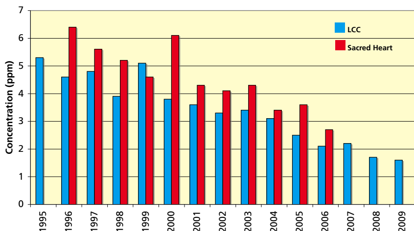
Carbon Monoxide Max. 8-Hr. Concentration
