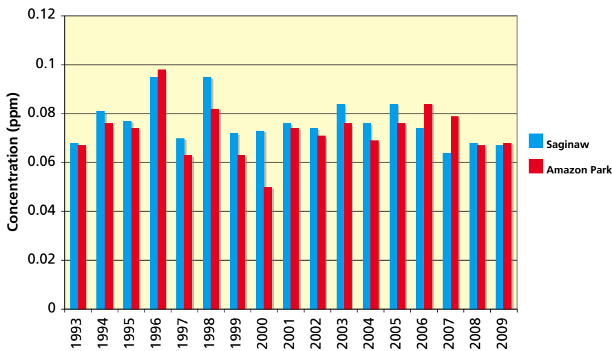
Ozone: Max. 8-Hr. Levels
