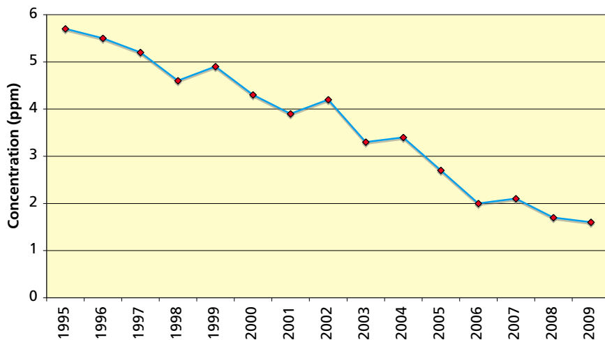
Yearly 8-Hr. Carbon Monoxide Levels: 2nd Highest Concentration
