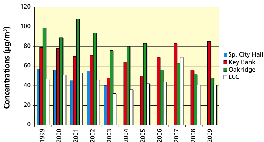
Particulate Matter (PM 10): Max. 24-Hr. Concentrations
